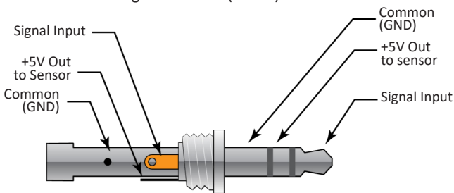
Figure 3 Input Connector Detail (stereo plug)
