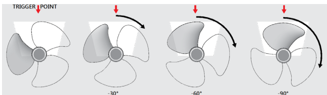
Figure 9 Phase Shifting by -30^\circ , -60^\circ , -90^\circ
