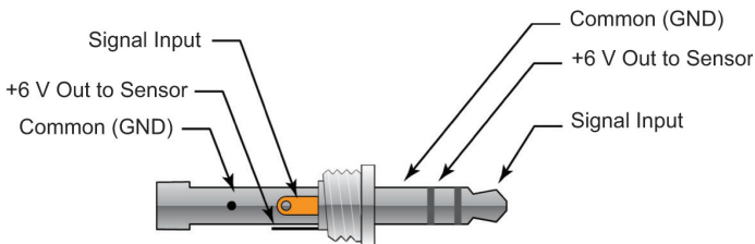
Figure 3 Output Connector Detail (Mono plug)
