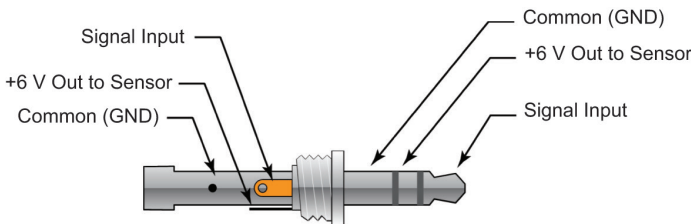
Figure 2 Input Connector Detail (Stereo plug)
